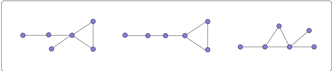
Figure 11: The three unlabelled Husimi graphs of molecular type y_2^3 y_3 \cdot X^4 E_2(X)
