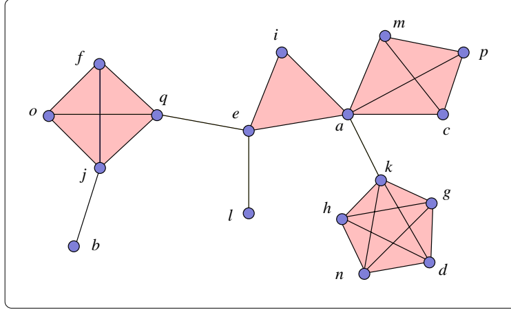
Figure 7: A Husimi graph with block-size distribution (4, 1, 2, 1, 0, \dots)
