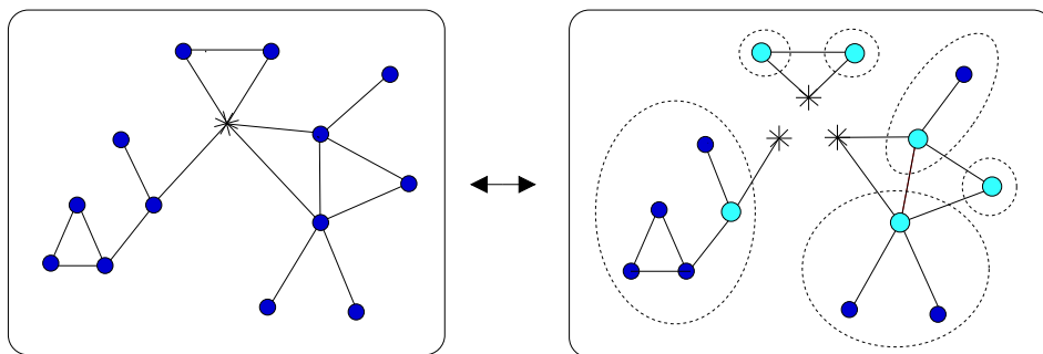
Figure 4: C'_{\mathcal{B}} = E(\mathcal{B}'(C_{\mathcal{B}}^\bullet))
