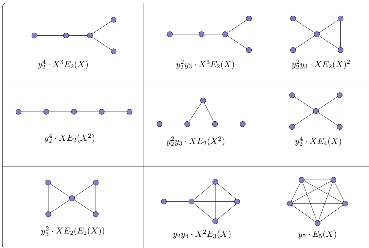
Figure 10: Husimi graphs of size 5
