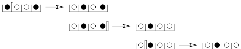
FIGURE 2. An example of evolution, with n = 4 . The active wall triggering each transition is indicated.
