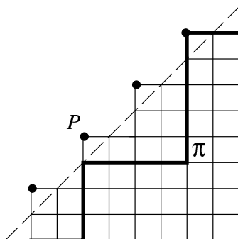
FIGURE 1. The path \pi = \underline{E} \underline{E} N N \underline{E} \underline{E} E E E N N N \underline{N} \underline{N} E E not above P = (N^2 E^2)^4 . It has i(\pi) = 3 and e(\pi) = 2 , corresponding to the steps underlined.
