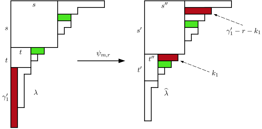
FIGURE 4. An example of the second symmetry bijection \psi_{m,r} : \lambda \mapsto \widehat{\lambda} , where \lambda \in \mathcal{H}_{n,m,\leq -r} , \widehat{\lambda} \in \mathcal{H}_{n',m+2,\geq -r} , for m = 0 , r = 2 , n = 92 , and n' = n - r - 2m - 2 = 88 . Here r_{2,0}(\lambda) = 2 + 2 - 9 = -5 \leq -2 and r_{2,2}(\widehat{\lambda}) = 3 + 4 - 6 = 1 \geq -2 , where \lambda = (14, 10, 9, 9, 8, 7, 7, 5, 4, 3, 3, 2, 2, 2, 2, 1, 1, 1) and \widehat{\lambda} = (13, 10, 9, 8, 8, 7, 6, 6, 5, 4, 3, 2, 2, 1, 1, 1, 1, 1) . Also, s = 7 , s' = s + 1 = 8 , s'' = s' - m - 2 = 6 , t = 3 , t' = 4 , t'' = 2 , \gamma'_1 = 9 , k_1 = 3 , and \gamma'_1 - r - k_1 = 4 .
