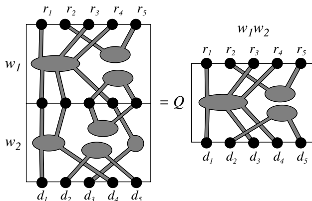
Figure 2: The product of seat-plans
