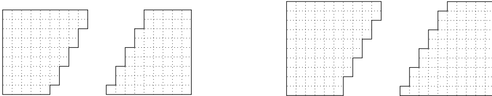
FIGURE 2. The boards of Lemma 3.8 for n = 9 (left) and n = 10 (right).
