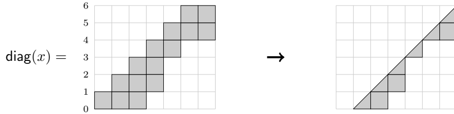
Fig. 2: On the left is shown P = \text{diag}(x) where x = (5, 5, 3, 2, 2, 1) \in \text{Rec}^\dagger(K_7) . The Dyck path \text{dyck}(P) = s^2 w^2 s w s^2 w s w^2 is shown on the right.
