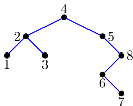
Fig. 6: The pruned tree for ((a_1 a_2)(a_3 a_4))a_5(a_6(a_7 a_8))a_9 labeled with the in-order labeling.
