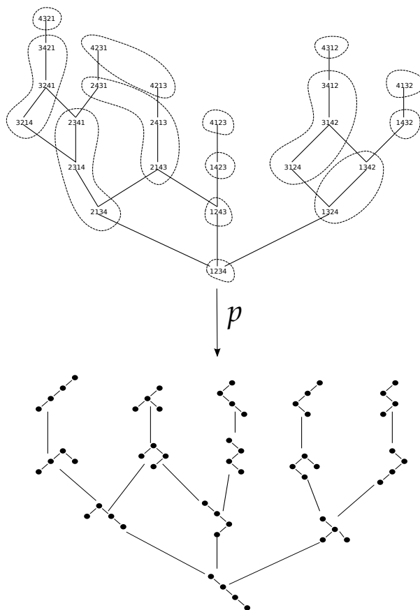
Fig. 8: The map p: \mathfrak{S}_4 \rightarrow \{\text{pruned trees with 4 vertices}\} .
