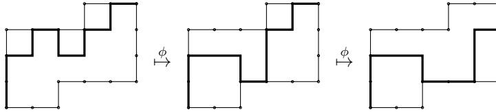
Fig. 4: The map \Phi applied to a path with two top contacts and no bottom contact. In this example, \phi first performs the transformation \phi_{[0,3]} , followed by \phi_{[3,5]} .
