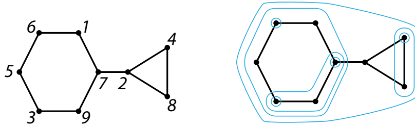
Fig. 2: (a) A graph G . (b) A nested set or tubing of G .
