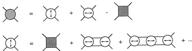
Fig. 5: Graphical representation of Eqs. (3.23) and (3.24).
