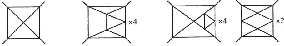
Fig. 6: The first contributions to \zeta[\Gamma] . All diagrams can be obtained from the ones depicted by rotations of 90 degrees.
