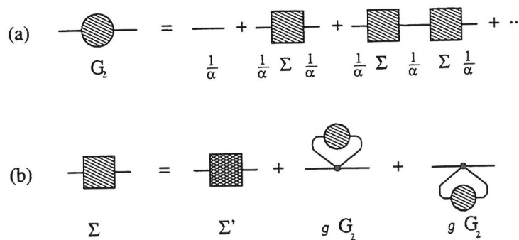
Fig. 3: (a): decomposition of the two-point function into its one-particle-irreducible part; (b) discarding one-vertex-reducible contributions
